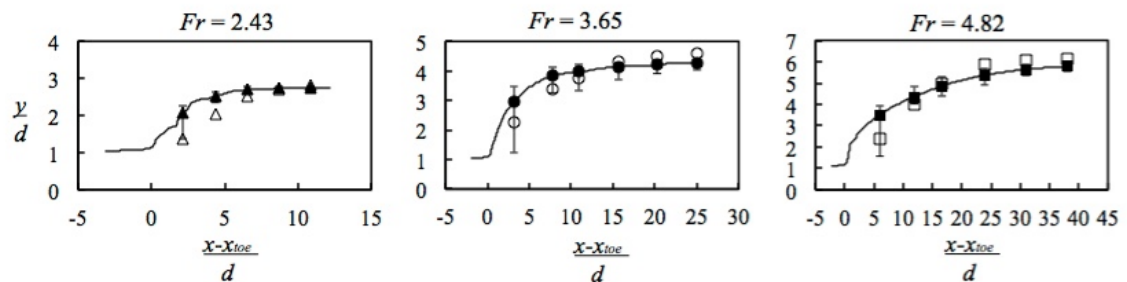
Figure 4.3. Mean free surface values from three simulations compared to experiments. Filled markers indicate simulation results while open markers indicate the elevation where \bar{\varphi} = 0.5 from Murzyn et al. (2005). Positive and negative error bars indicate simulation elevations with \bar{\varphi} = 0.2 and \bar{\varphi} = 0.8 , respectively.
