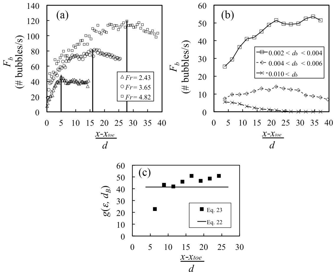
Figure 4.24. (a) Flux of bubbles downstream for all jumps. Solid black line indicates \max F_b . (b) Flux of bubbles downstream by bubble size for Fr = 4.82 . (c) Comparison of breakup frequency in the roller region for Fr = 4.82 , d_b > 0.01 m.
