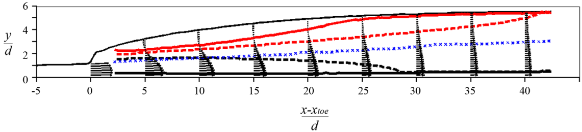
Figure 4.13. Mean velocity components for Fr = 4.82 compared with the mean shear layer elevation, \bar{y}_s . Upper and lower solid lines indicate minimum and maximum positive \bar{u}_x , respectively, upper and lower dashed lines represent \bar{u}_x = 0.35 U_o and \bar{u}_x = 0.1 U_o , respectively, and the center 'x' indicates \bar{y}_s .
