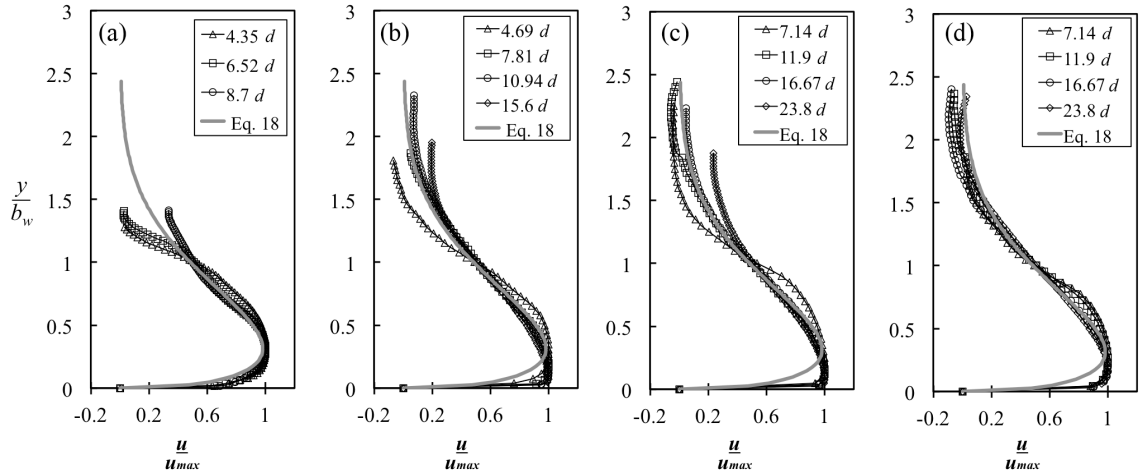
Figure 3.5. Time-averaged velocity profile compared to a wall-jet similarity solution for Fr = 2.43 (a), Fr = 3.65 (b), Fr = 4.82 2D (c), and Fr = 4.82 3D (d).
