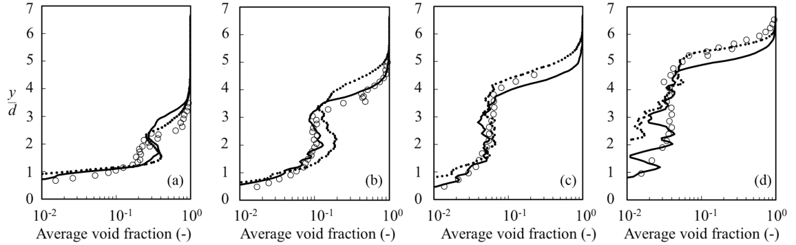
Figure 3.9. Average void fraction profiles for Fr = 4.82 at x-x_{toe} = 7.14d (a), 11.9d (b), 16.67d (c), and 23.8d (d). ‘ \circ ’ denotes experimental average void fraction (Murzyn, 2013); ‘- - -’ denotes 2D simulated average void fraction; ‘—’ denotes 3D simulated average void fraction.
