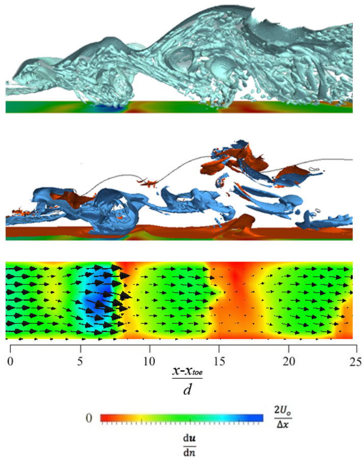
Figure 4.17. Instantaneous depiction of lower wall shear, du/dn . Top: three-dimensional isosurface of volume fraction about \gamma = 0.95 to represent bubbles. Middle: three-dimensional isosurface of \omega_z = 0.4d/U_o (blue) and \omega_z = -0.4d/U_o (orange) along with a solid black contour of \gamma = 0.5 to represent the free surface. Bottom: top view of lower wall colored by du/dn with velocity vectors indicating direction of motion in the grid node above the wall.
