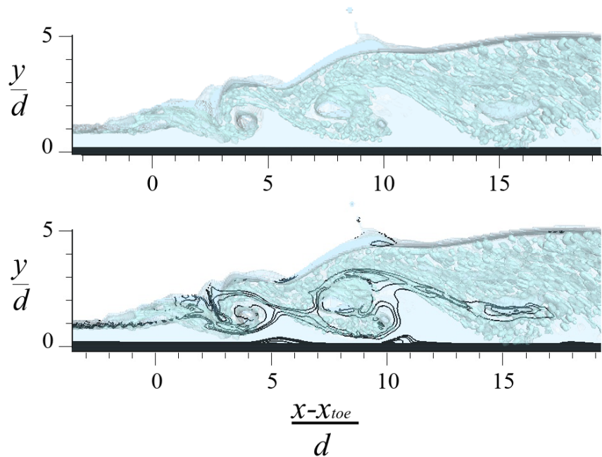
Figure 3.22. Selected instantaneous vorticity contours (black lines) for \omega_{mag} = 30, 40, 50, 100, 200 \text{ s}^{-1} , through a 2D x - y plane down the center of the domain, and bubbles represented by a volume fraction isosurface on \gamma = 0.95 , during a roll-up of a streamwise vortex (from Figure 3.191). Top: spatially inhomogeneous bubble field. Bottom: a lack of bubbles is seen on the lower downstream side spanwise vortices, below the location of streamwise vortex pairs, and above the region where vorticity is shed from the wall.
