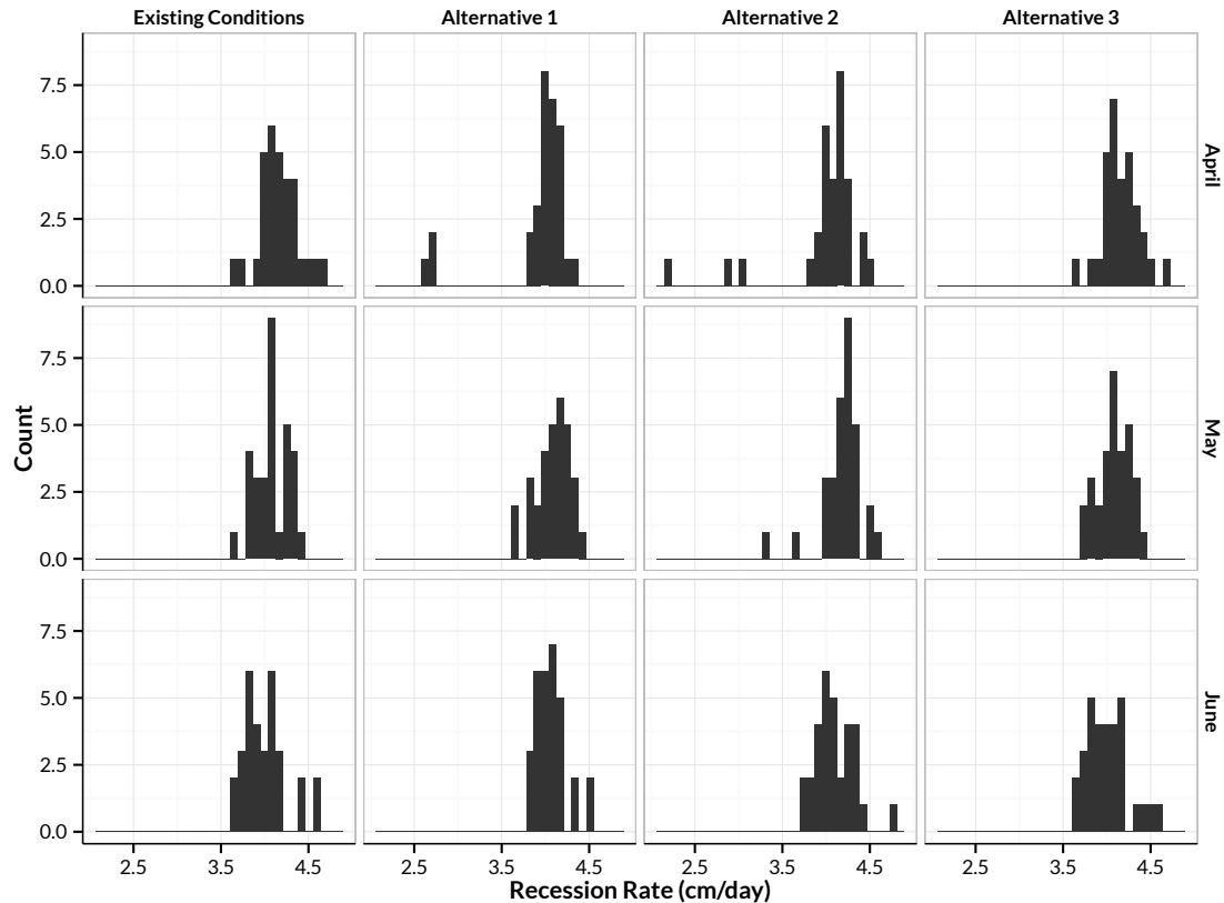
Figure 3.6: Histograms for mean daily river stage recession rate faceted by alternative and month.
