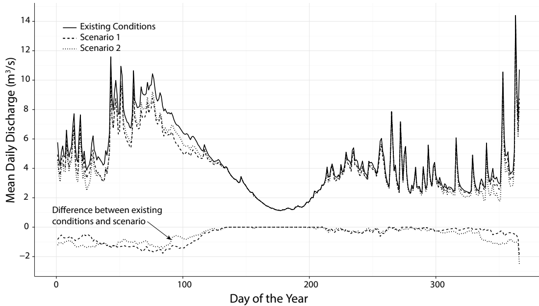
Figure 4.2: Mean daily discharge for existing conditions and the diversion scenarios between August 30, 1935 and August 6, 2013. Data for existing conditions originated from USGS gage 09430500. Also illustrated are the mean daily differences in discharge between existing conditions and each scenario.
